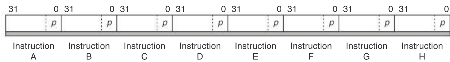
Figure E.6 Instruction packet of the TMS320C6x family of DSPs. The p bits determine whether an instruction begins a new VLIW word or not. If the p bit of instruction i is 1, then instruction i + 1 is to be executed in parallel with (in the same cycle as) instruction i . If the p bit of instruction i is 0, then instruction i + 1 is executed in the cycle after instruction i . (Courtesy Texas Instruments.)
