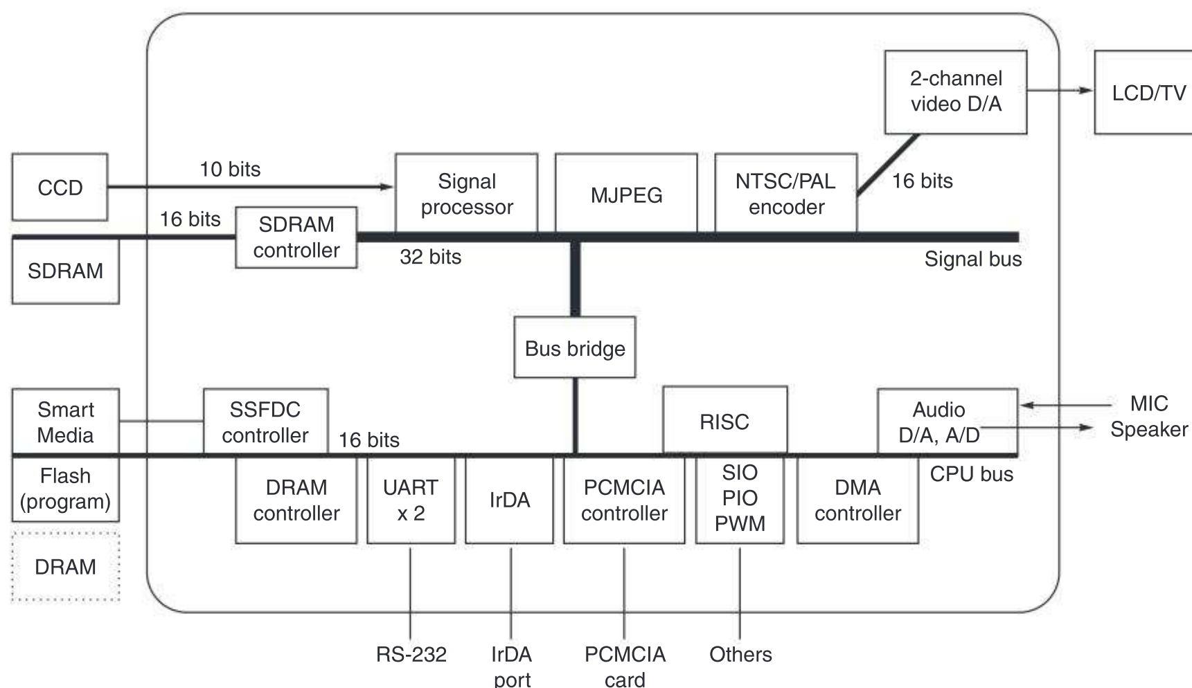
Figure E.13 The system on a chip (SOC) found in Sanyo digital cameras. This block diagram, found in Okada et al. [1999] , is for the predecessor of the SOC in the camera described in the text. The successor SOC, called Super Advanced IC , uses three buses instead of two, operates at 60 MHz, consumes 800 mW, and fits 3.1M transistors in a 10.2 \times 10.2 mm die using a 0.35-micron process. Note that this embedded system has twice as many transistors as the state-of-the-art, high-performance microprocessor in 1990! The SOC in the figure is limited to processing 1024 \times 768 pixels, but its successor supports 1360 \times 1024 pixels.
