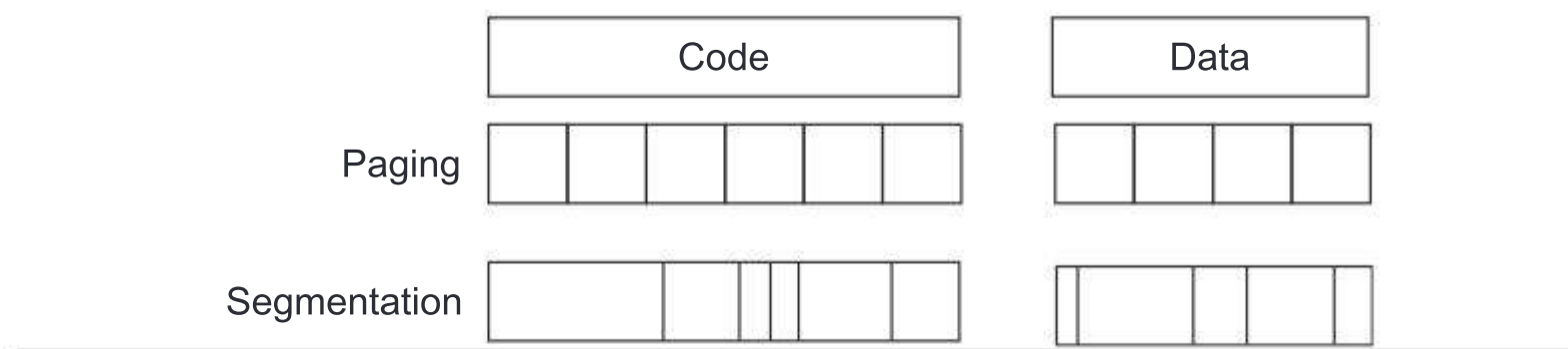
Figure B.21 Example of how paging and segmentation divide a program.
